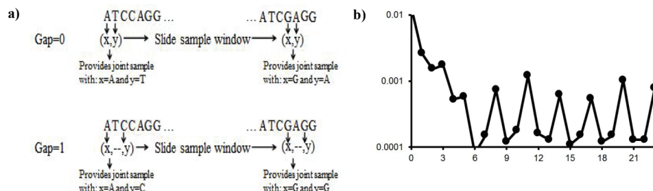
Figure 1: Codon structure is revealed in the V. cholera genome by mutual information [13] between nucleotides in the genomic sequence when evaluated for different gap sizes.
